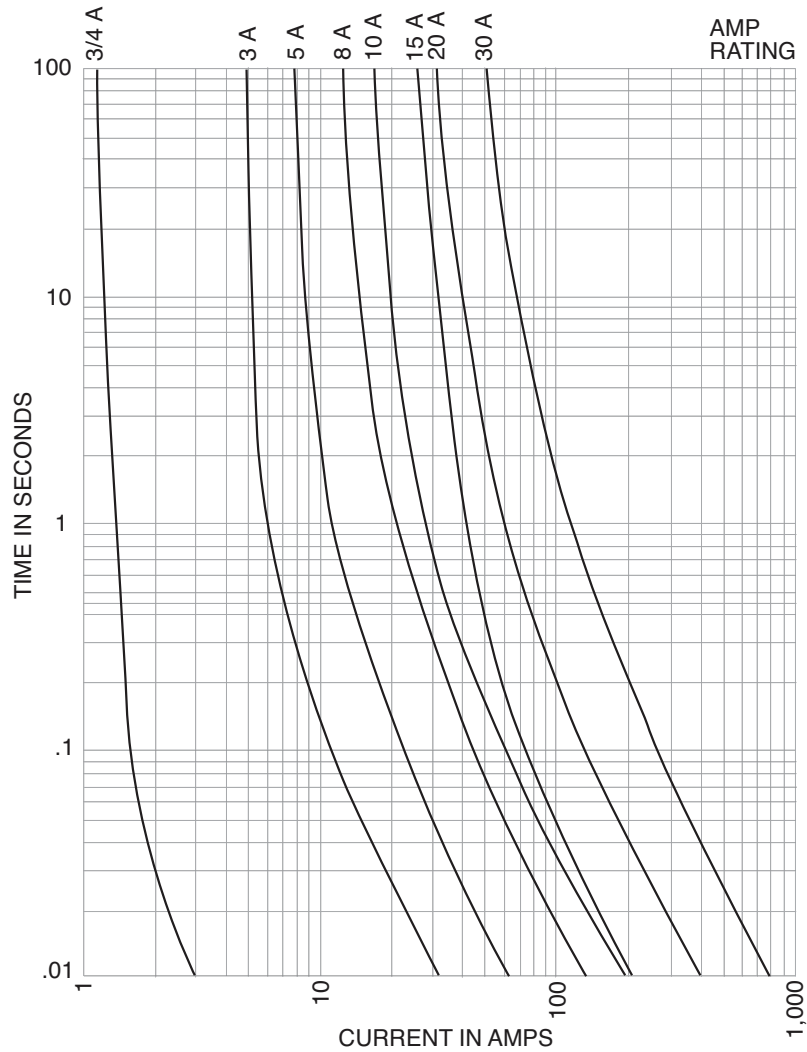
Time Curve for the KLM Fuse
